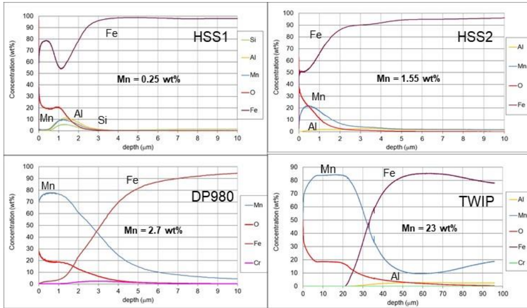
Fig. 2: GDOES quantitative depth profiles of the steel samples after oxidation at 900°C in 7% H 2 -N 2 with DP of -20°C
