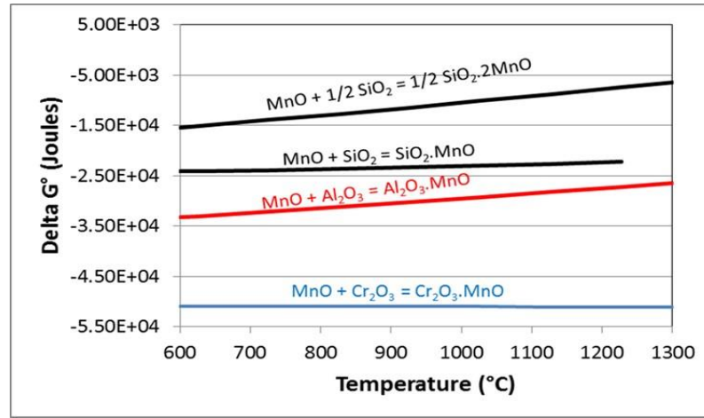
Fig. 4: Values of Gibbs energy change of MnO reactions with pure oxides (ThermoCalc®, SSUB3 module).
