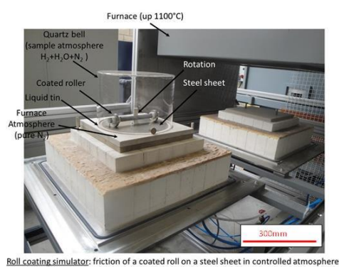
Fig. 1: NoStickRoll (NSR) equipment developed for the pick-up study and example of thermal cycle applied with sequential friction at 7 turns/min (blue section).
