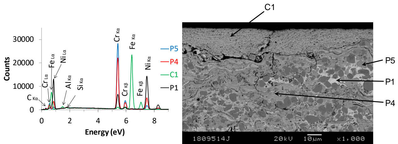
Fig. 9: SEM mapping in cross section under a pick-up from HSS2.
