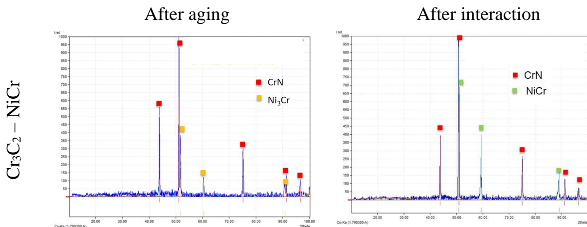
Fig. 7: XRD results of \text{Cr}_3\text{C}_2\text{-NiCr} based matrix coatings after ageing and after interaction with TWIP steel at DP-40°C.
