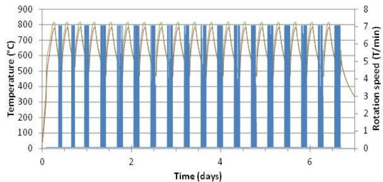
Fig. 1: NoStickRoll (NSR) equipment developed for the pick-up study and example of thermal cycle applied with sequential friction at 7 turns/min (blue section).
